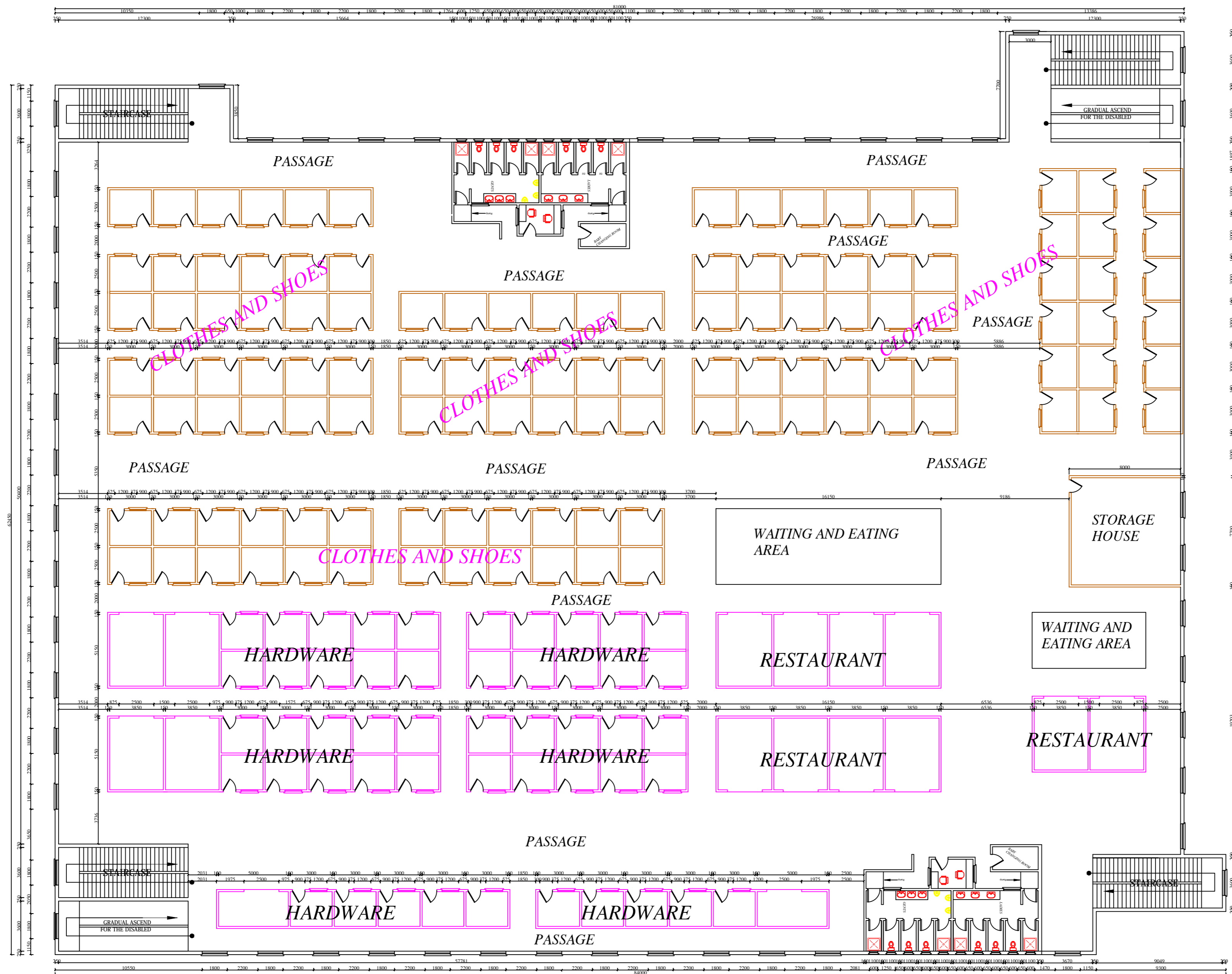
FLOOR PLAN FIRST FLOOR
