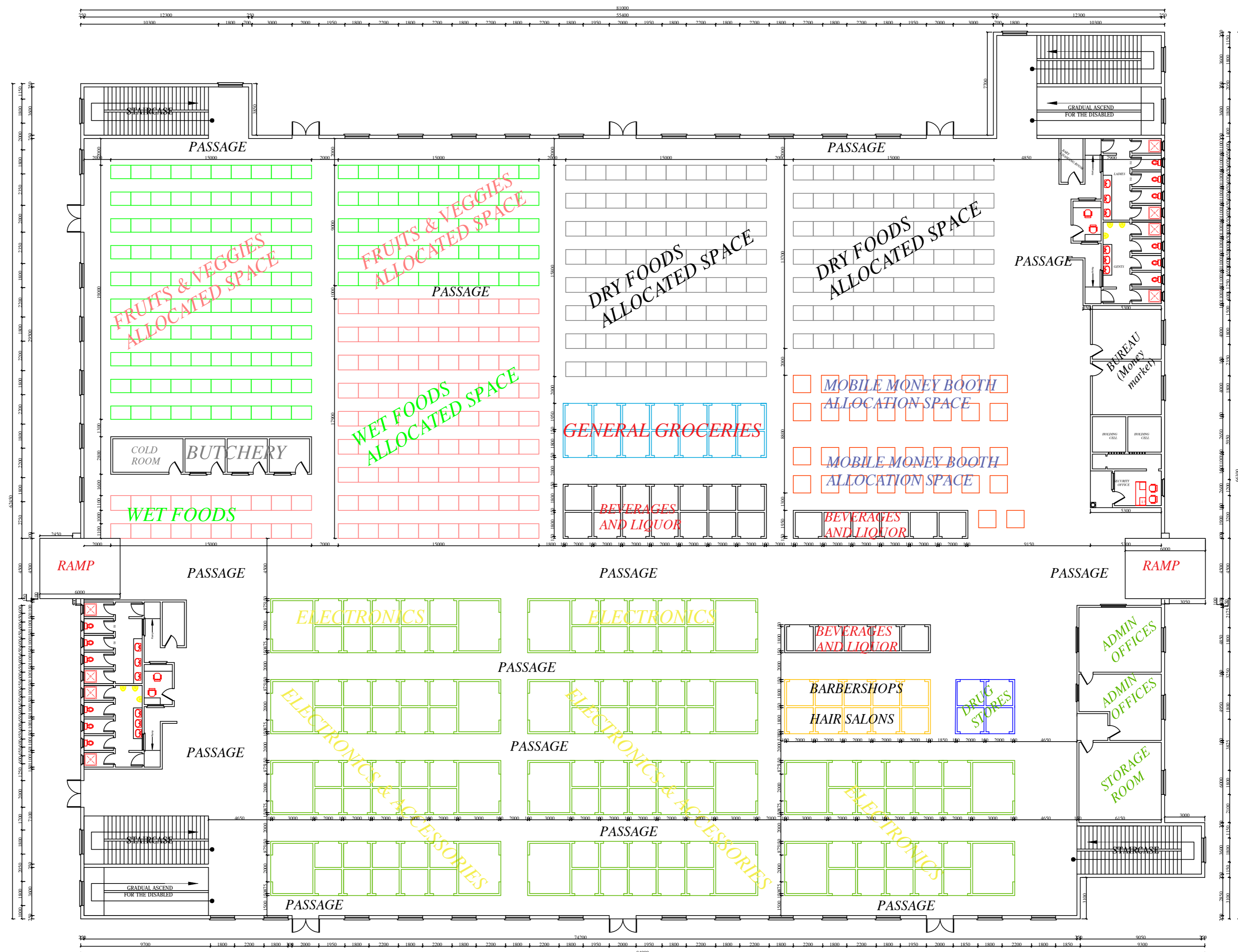
FLOOR PLAN GROUND FLOOR
