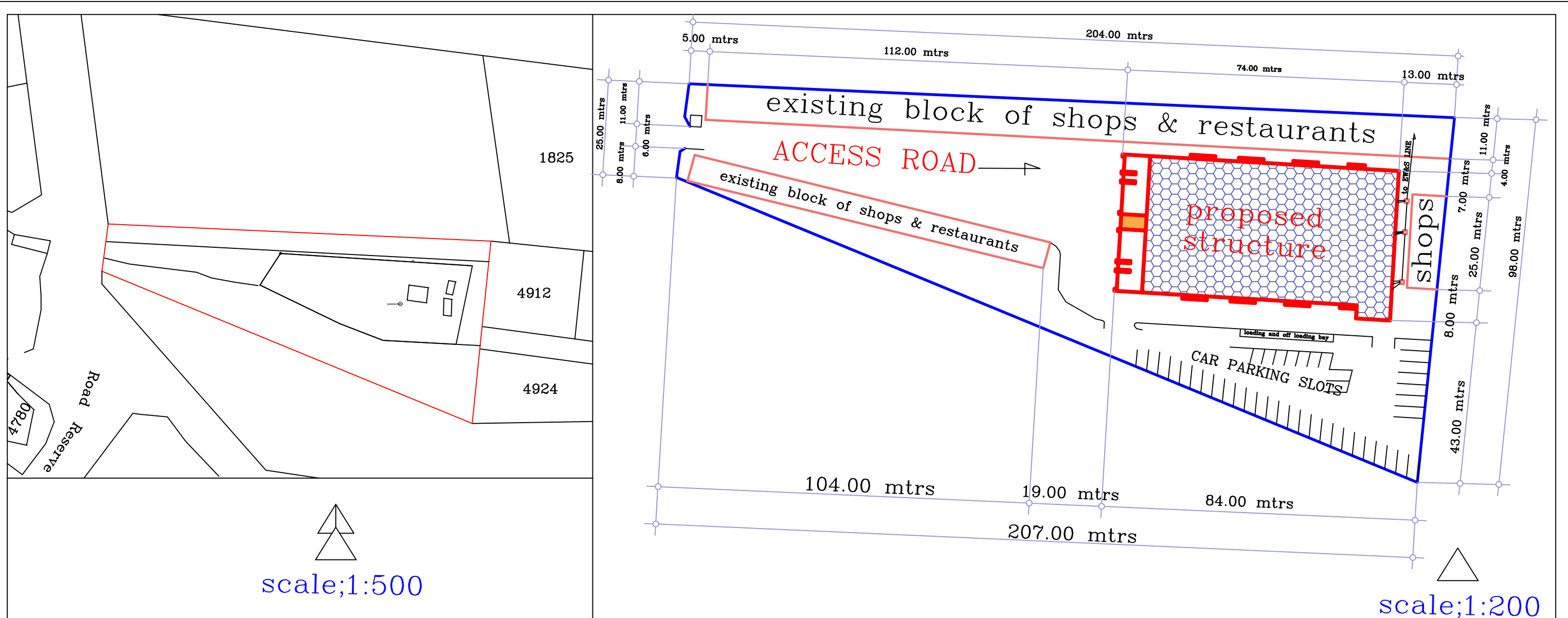
CHIPATA: PROPOSED SITE AND BLOCK PLAN SHOWING CROSS BORDER MARKET-CHIPATA FOR CROSS BORDER TRADER ASSOCIATION (CBTA)- CHIPATA ON PLOT No. 4766
